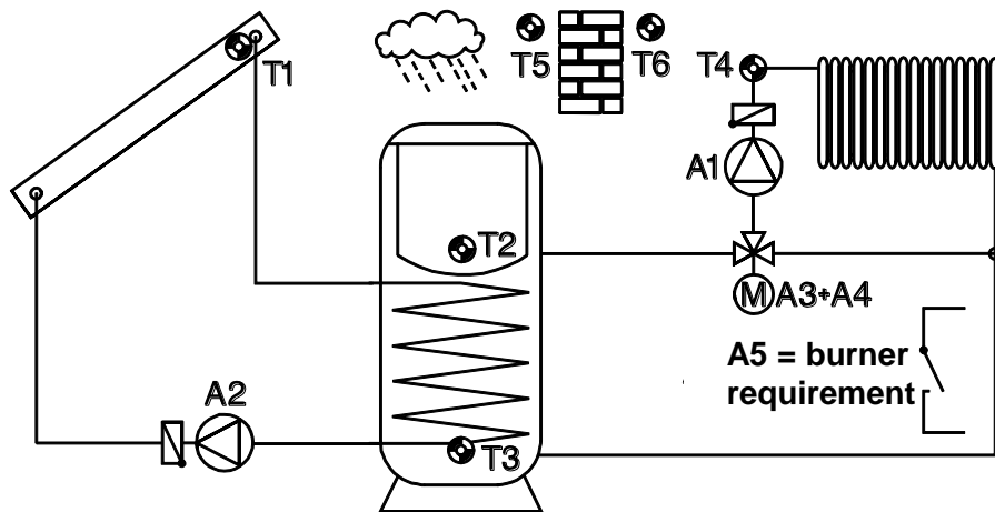
Diagram 80: Solar power unit, (combined) buffer tank, heating circuit, burner requirement
