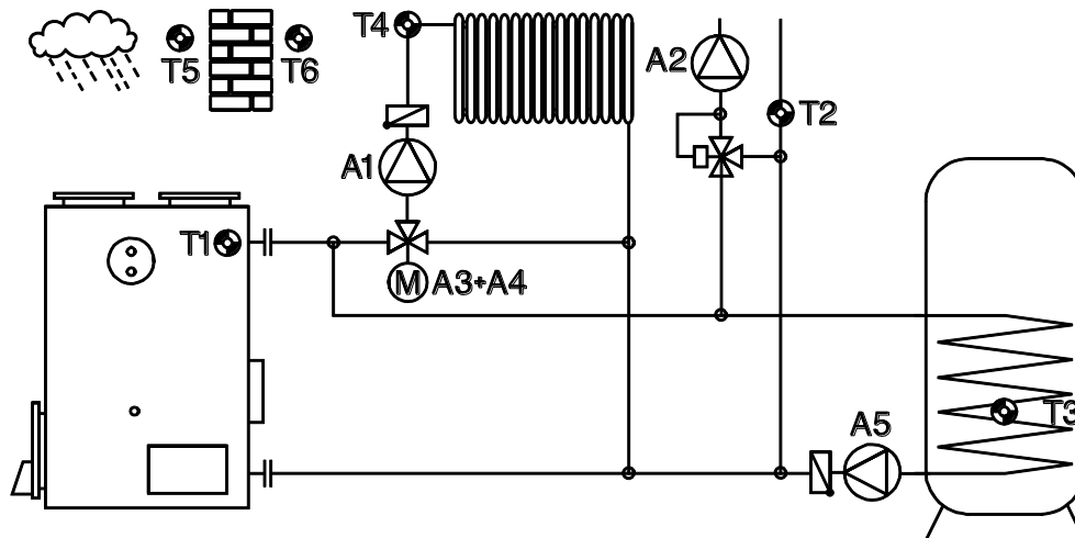
Diagram 96: Boiler (or buffer tank), hot water tank, 2 heating circuits
