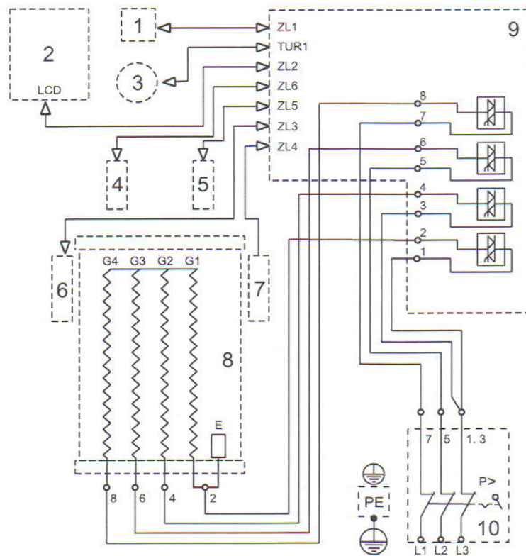
Fig. 7 Schematic diagram of POW-LCD MULTI
